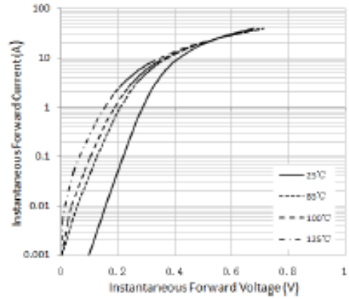
Figure 2. Typical Instantaneous Forward Characteristics
