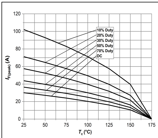
Fig.3 -Current Derating
